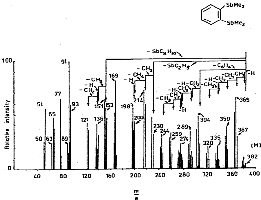
Figure 1. Diagram of mass spectrum of o -phenylenebis (dimethylstibine). E. Shewchuk and S.B. Wild, Synthesis of o -phenylenebis(dimethylstibine) and some derivatives of divalent nickel, palladium, and platinum and of zerovalent chromium, molybdenum and tungsten.
